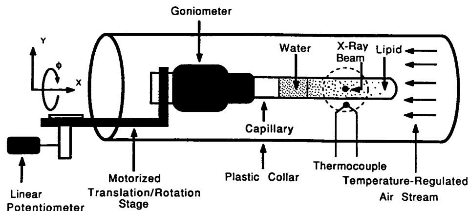
FIGURE 1 Schematic diagram of the experimental arrangement for time-resolved x-ray diffraction from lyotropic gradient samples. See text for details.
